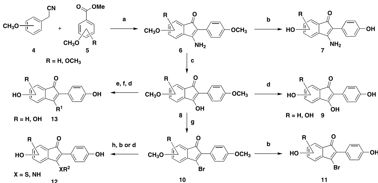
Scheme 1. Reagents and conditions: (a) LDA, THF, −10 °C; (b) BBr 3 , CH 2 Cl 2 ; (c) 20% H 2 SO 4 , 100 °C; (d) pyridine–HCl; 180 °C; (e) NaHMDS, THF, 0 °C; (f) R 1 MgBr or R 1 Li, THF, 0 °C–rt; R 1 = Me, Ph; (g) CBr 4 , PPh 3 , CHCl 3 ; (h) R 2 –NH 2 or R 2 –SNa, DMF, 60–80 °C; R 2 = Me, Et.
